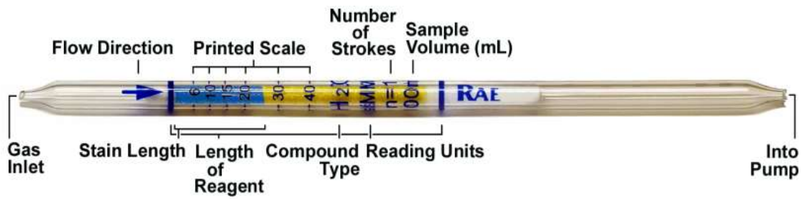
Figure 19 – Gas Detection Tube
