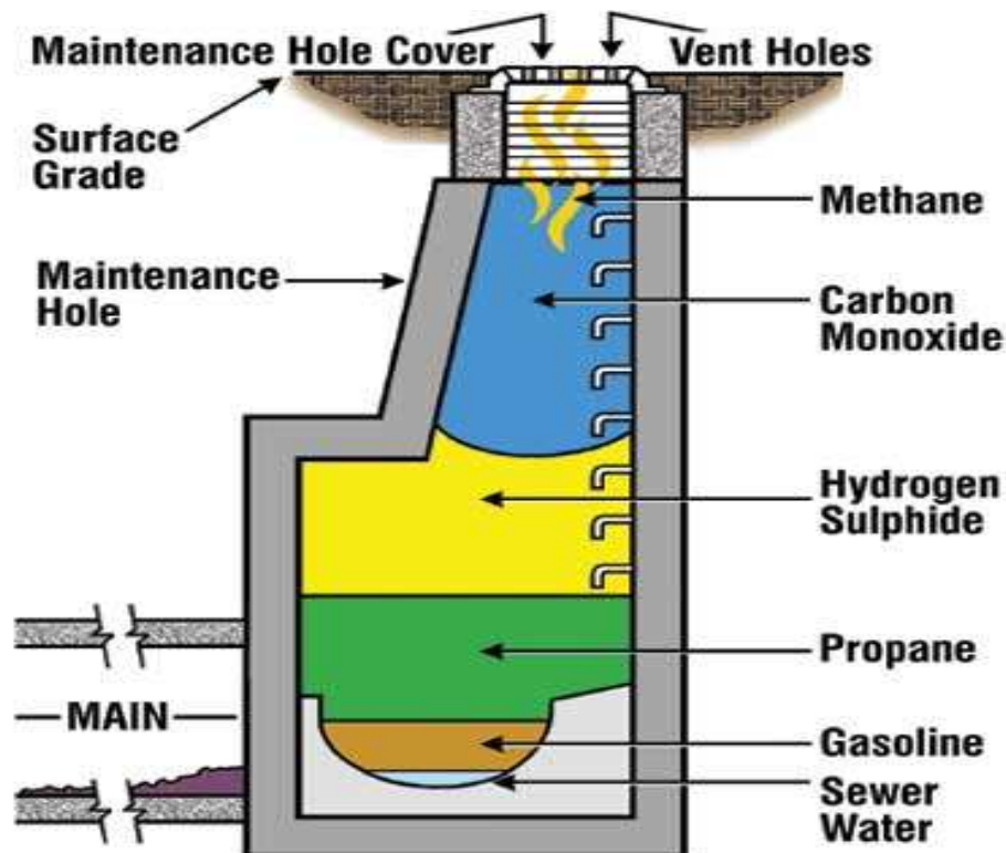
Figure 3 – Gas density layering
