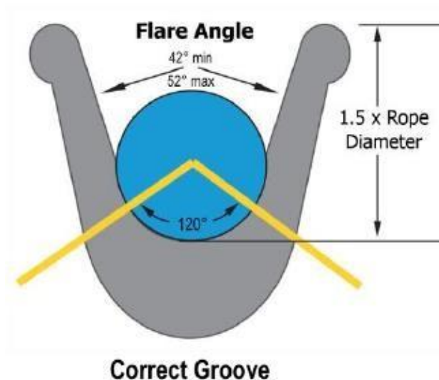
Figure 10 – Sheave angle
