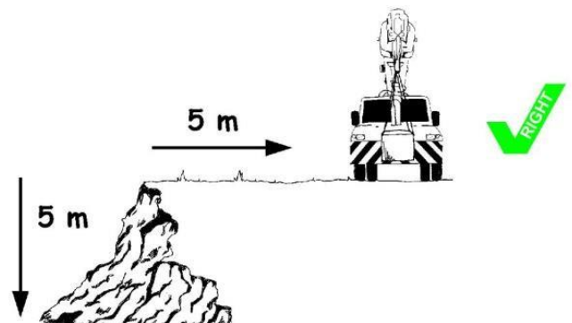
Figure 18 – Excavation Distance
