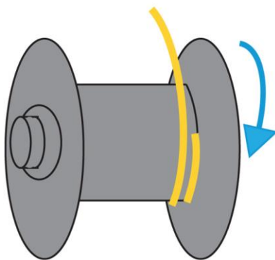
RL Lay Rope Overwound
